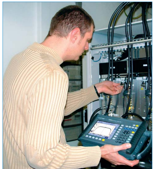
Channel power measurements at a UMTS Node B
